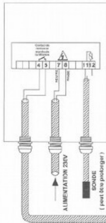
COFFRET GELELEC'
